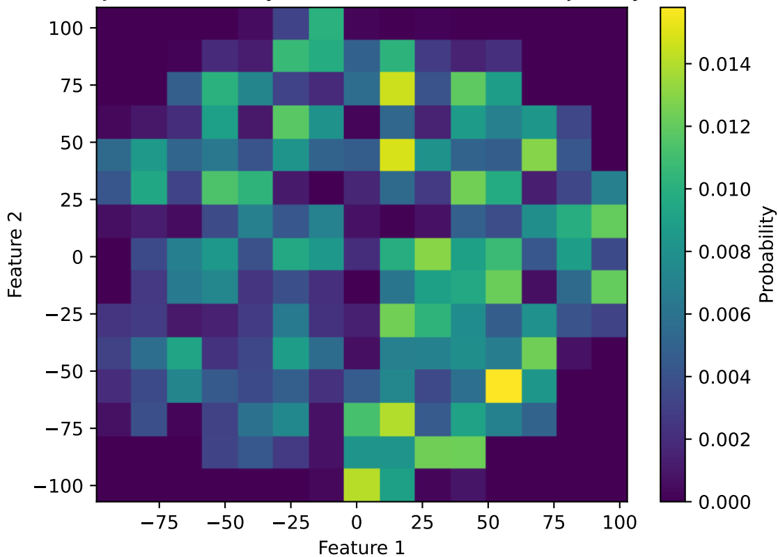
t-SNE Joint Probability Distribution for DDPM Trajectory Set
