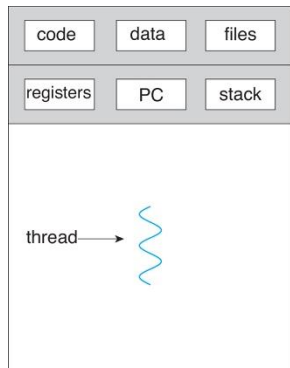
single-threaded process
