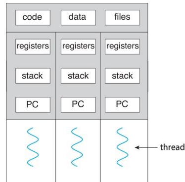
multithreaded process
