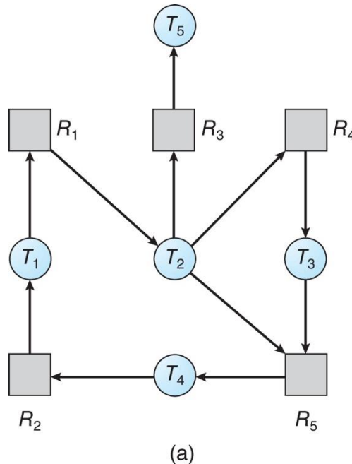
Resource-Allocation Graph
