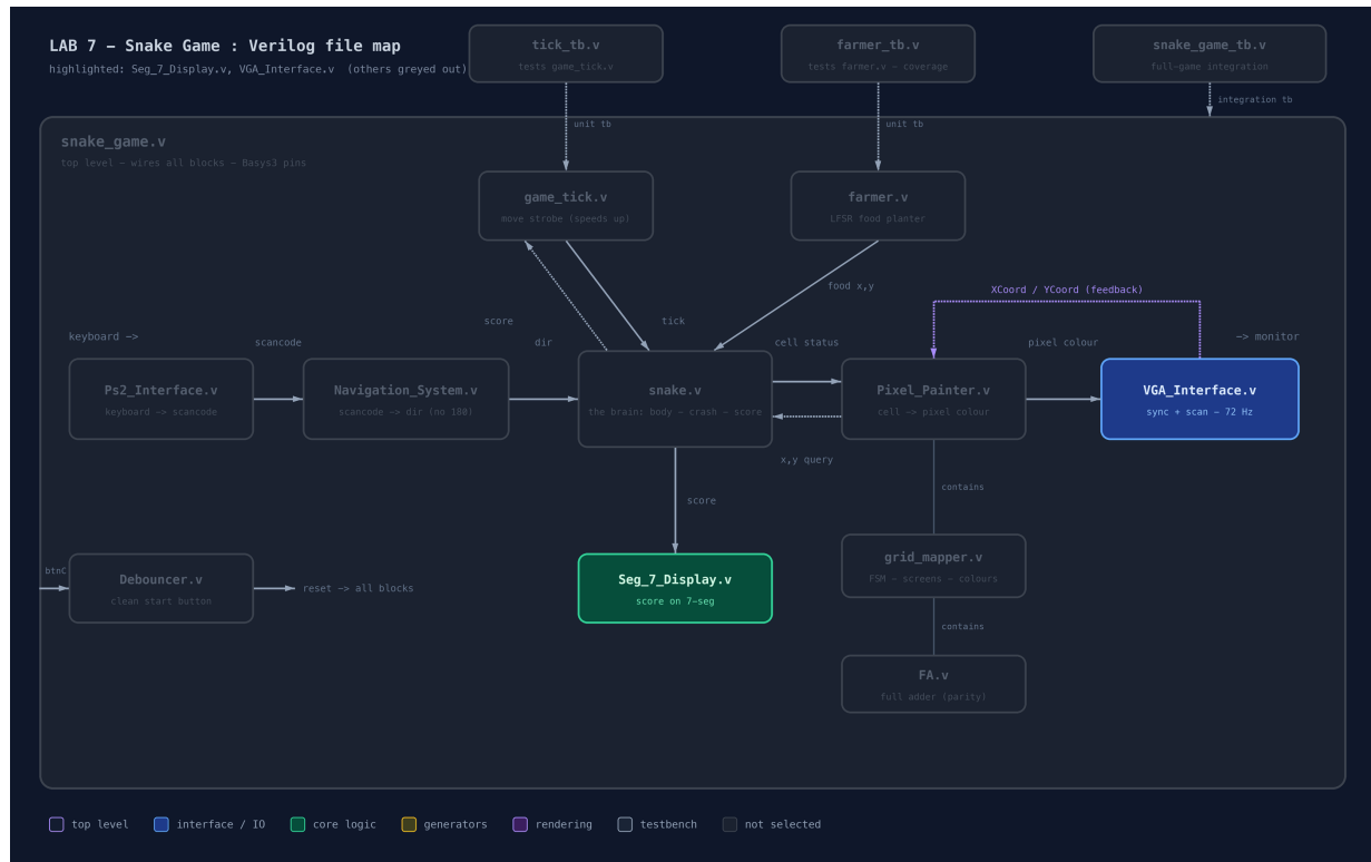
Figure 9: Output block highlighted.
