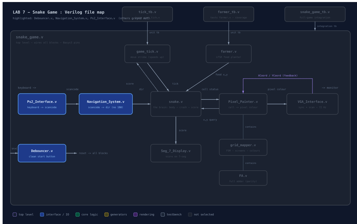
Figure 3: Input and control block highlighted.
