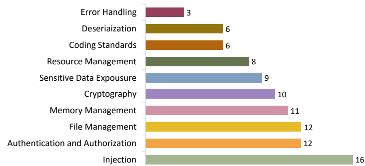
Fig. 2. Bar chart showing the number of studies discussing each category of security vulnerabilities introduced by LLMs.
