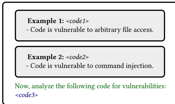
Fig. 5. Example of a prompt, using the few-shot prompting technique. In the gray boxes, the code examples and corresponding vulnerabilities provided to the LLM. In green, the main body of the instructions. In blue, the code to be analyzed.
