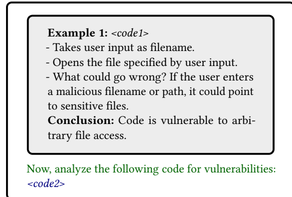
Fig. 6. Example of a prompt, using the CoT prompting technique. In the gray boxes, the code example and the reasoning steps provided to the LLM. In green, the main body of the instructions. In blue, the code to be analyzed.
