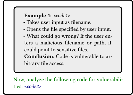
Fig. 13. Example of a prompt, using the CoT prompting technique. In the gray boxes, the code example and the reasoning steps provided to the LLM. In green, the main body of the instructions. In blue, the code to be analyzed.
