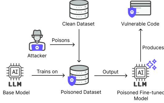
Fig. 14. Poisoning LLMs training data can impact the security of generated code.
