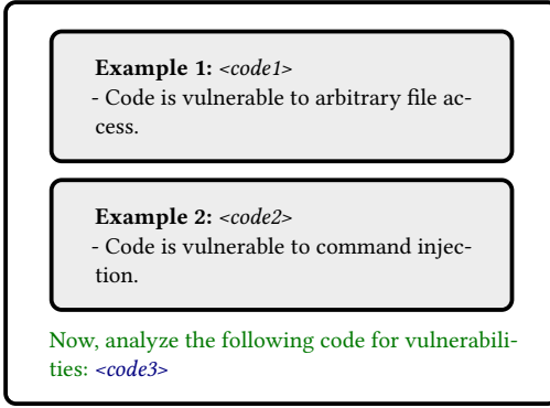
Fig. 12. Example of a prompt, using the few-shot prompting technique. In the gray boxes, the code examples and corresponding vulnerabilities provided to the LLM. In green, the main body of the instructions. In blue, the code to be analyzed.
