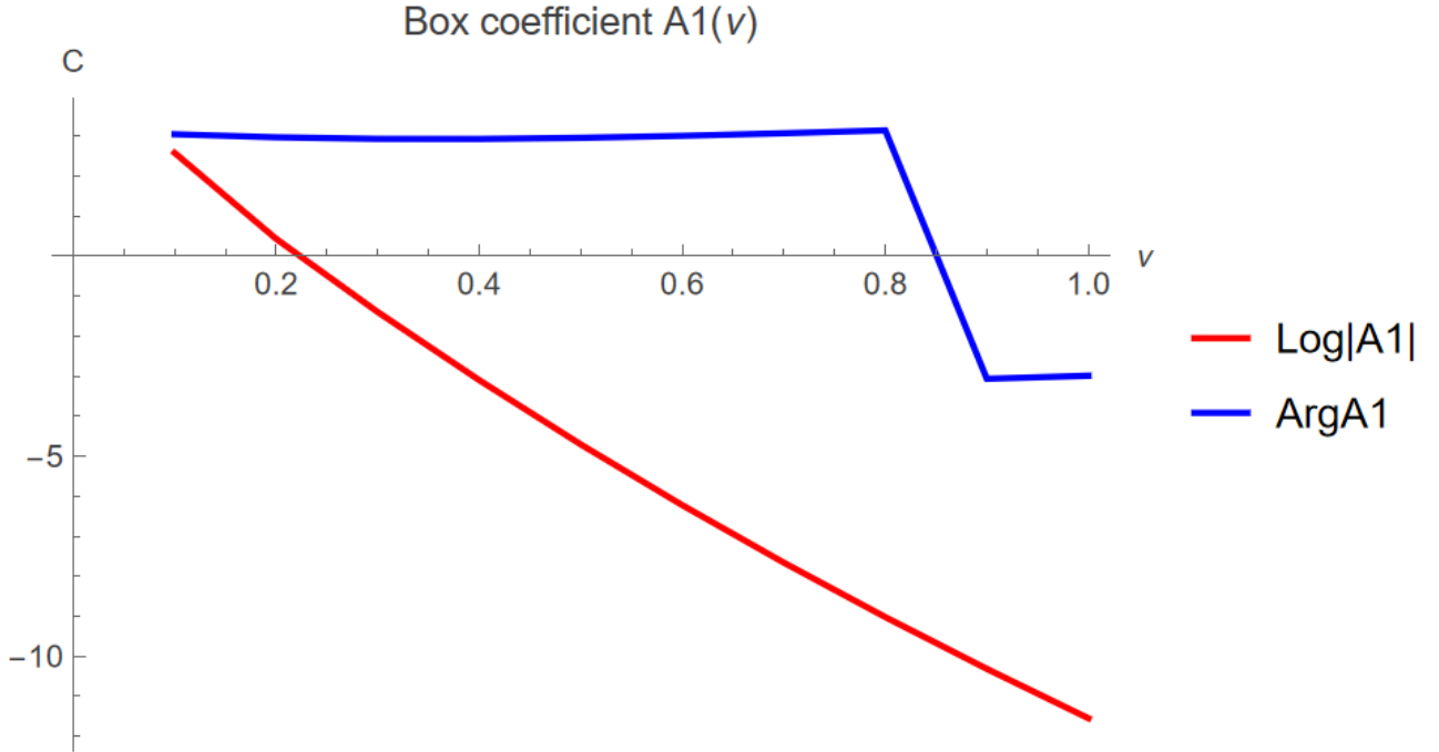
Figure 3: A_1(\tilde{\nu})
