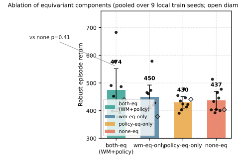
Figure 4: Ablation of equivariant components pooled over nine local train seeds. Error bars are 95% confidence interval; dots are individual local seeds; the open diamond is the pooled two-seed A10 cloud cross-check. No configuration is significantly better: the paired both-eq vs none-eq difference is +37 with p = 0.41 .
