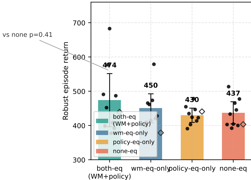
Ablation of equivariant components (pooled over 9 local train seeds; open diamond)
