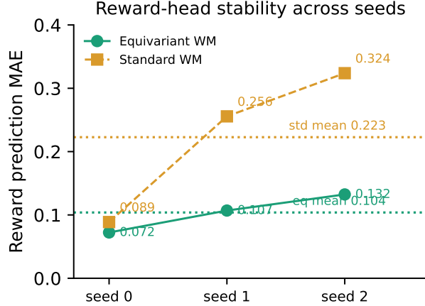
Figure 2: Per-seed reward-prediction MAE. The equivariant reward head stays in [0.072, 0.132] across seeds, whereas the non-equivariant head diverges on two of three seeds (0.256, 0.324). The benefit is cross-seed stability , not a uniformly large per-sample accuracy gain.
