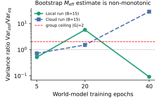
Figure 5: Bootstrap estimate of the effective multiplier (variance ratio, log scale) versus world-model training epochs. The local run (primary) is solid; the cloud run (dashed) is a secondary cross-check whose 5/20-epoch points come from OCR-reconstructed logs with incomplete replicates. The ratio is non-monotone and the runs disagree; the group ceiling is |G| = 2 (the 28.3 cloud value is raw, clipped to 2.0). We treat any multiplier above 1 as unconfirmed.
