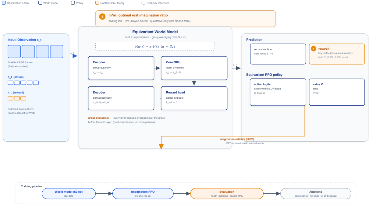
Figure 1: Overview of the equivariant world model and imagination training. The world model enforces hard Z_2 equivariance by group averaging across an Encoder, a ConvGRU dynamics cell, a Decoder, and a reward head; it predicts both frame reconstruction and a scalar reward. The equivariant PPO policy is updated inside the learned model on imagination rollouts, and the analysis bounds the optimal real:imagination ratio m^*/n only qualitatively.
