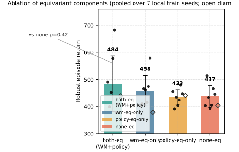
Figure 4: Ablation of equivariant components pooled over seven local train seeds. Error bars are 95% confidence intervals; dots are individual local seeds; the open diamond is the pooled two-seed A10 cloud cross-check. No configuration is significantly better: the paired both-eq vs none-eq difference is +47 with p = 0.42 .
