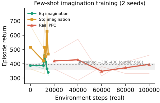
Figure 3: Few-shot imagination training (2 seeds). Thin lines are individual seeds, thick lines their mean. Imagination agents at \sim 15 k real steps match real PPO evaluated at 20k–40k steps. The gray band marks the untrained-policy range ( \sim 380 –400; one outlier seed at 668); all curves are noisy at this budget.
