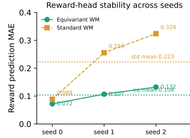
Figure 2: Per-seed reward-prediction MAE. The equivariant reward head stays in [0.072, 0.132] across seeds, whereas the non-equivariant head diverges on two of three seeds (0.256, 0.324). The benefit is cross-seed stability , not a uniformly large per-sample accuracy gain.
