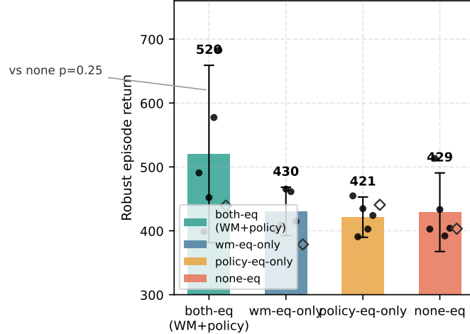
Ablation of equivariant components (pooled over 5 local train seeds; open diam
