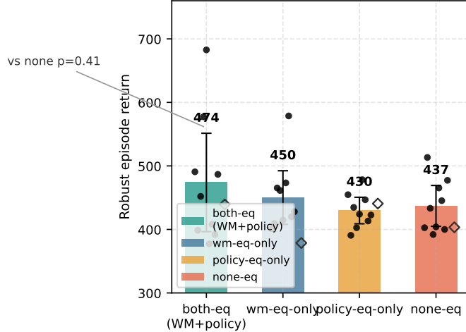
Ablation of equivariant components (pooled over 9 local train seeds; open diam
