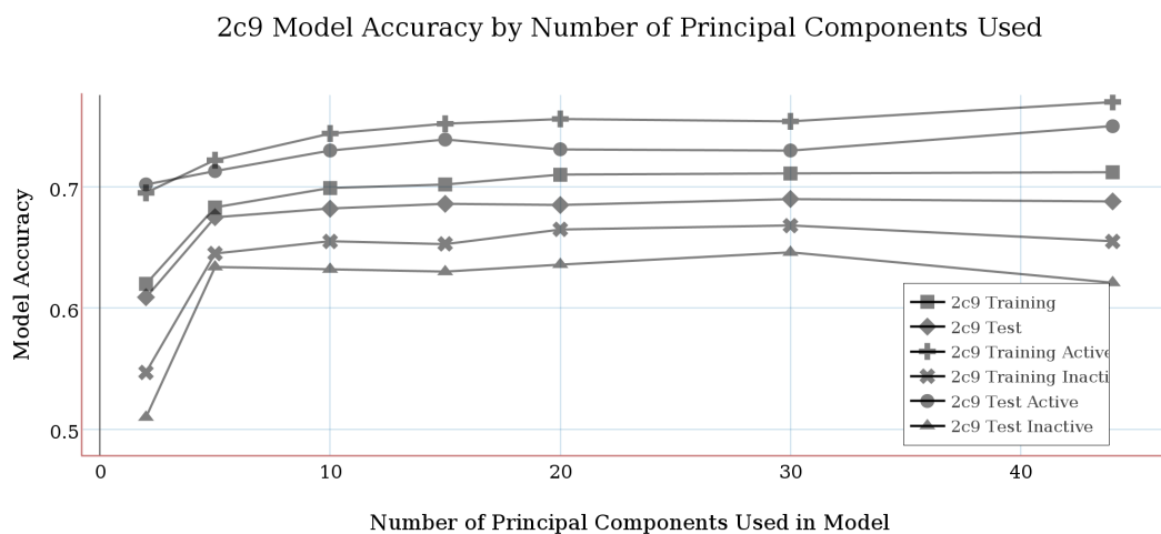
Figure 3.2: 2C9 MOE Model Accuracy
