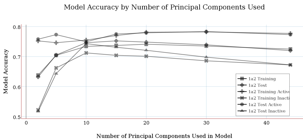
Figure 3.1: 1A2 MOE Model Accuracy
