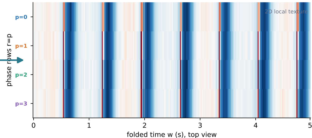
B. Same samples: CNN top view after P=4
