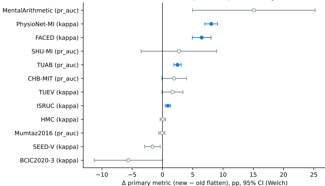
Effect sizes with 95% confidence intervals (filled = Holm-corrected p < .05 , open = not significant)
