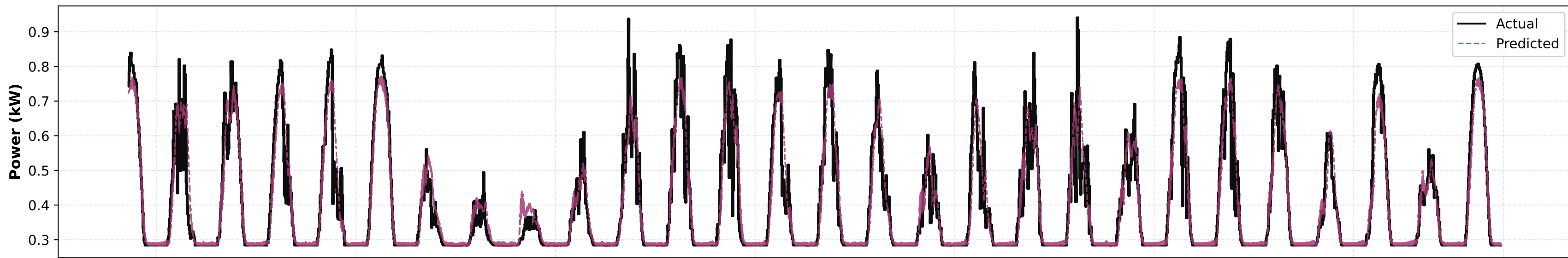
Bozhou PV - H=16 (4-hour Forecast) | RMSE=0.0713, MAE=0.0409, R2=0.8057
