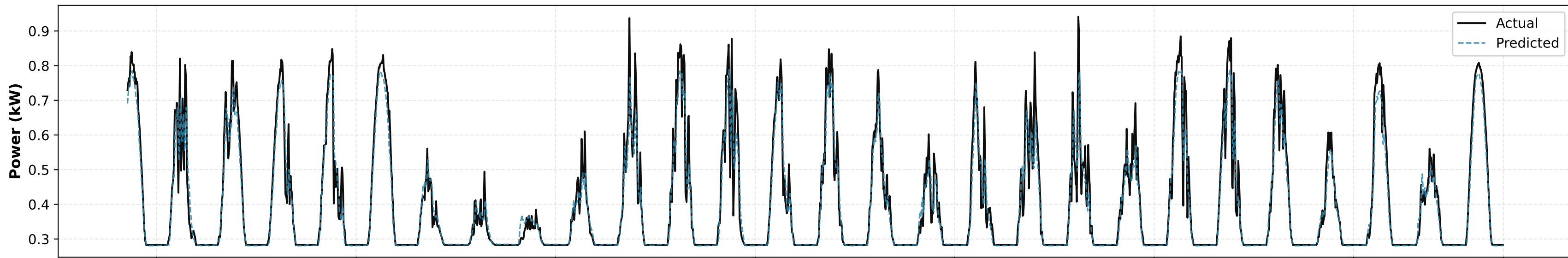
Bozhou PV - H=4 (1-hour Forecast) | RMSE=0.0595, MAE=0.0331, R2=0.8652
