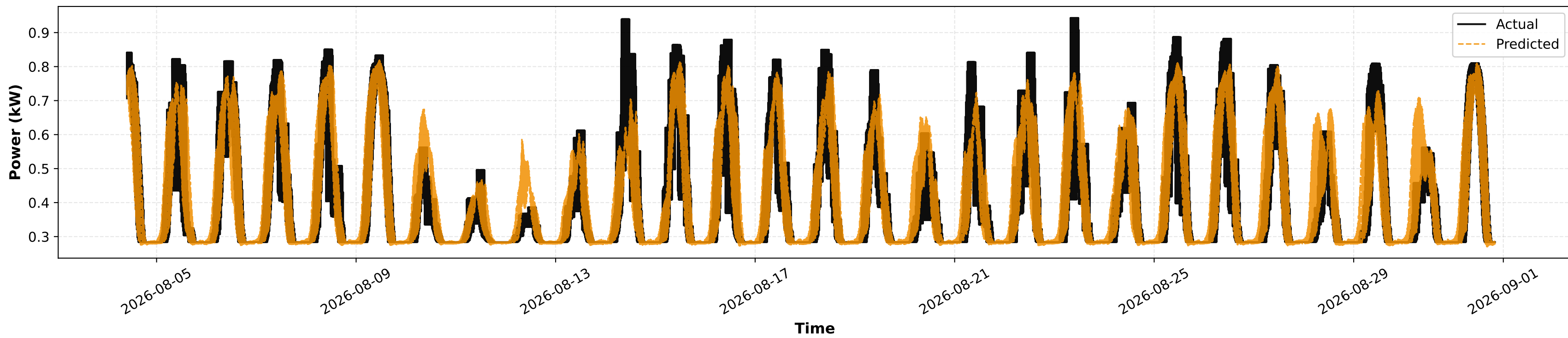
Bozhou PV - H=16 (4-hour Forecast) | RMSE=0.0713, MAE=0.0409, R2=0.8057
