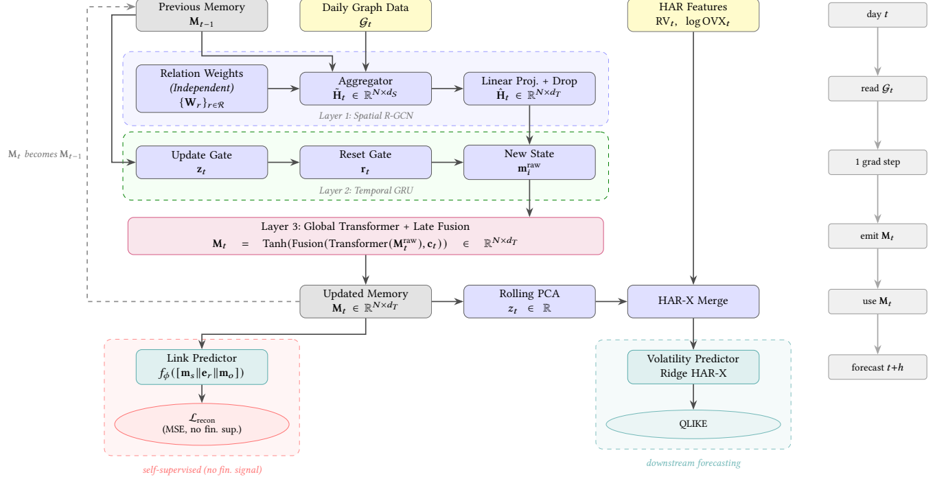
Figure 1: Proposed spatio-temporal graph autoencoder. The encoder stacks three hierarchical layers (Spatial R-GCN \rightarrow Temporal GRU \rightarrow Global Transformer) followed by a late fusion mechanism. The self-supervised link-prediction head ( \mathcal{L}_{recon} ) receives no financial supervision, decoupling geopolitical representation learning from the downstream Ridge HAR-X forecasting head (QLIKE). Right panel: strict online protocol.
