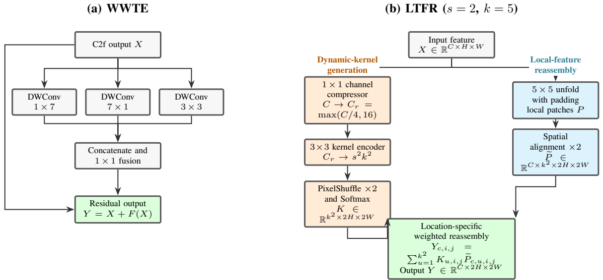
Fig. 4. Internal structures of (a) WWTE and (b) LTFR. WWTE uses three depthwise branches and residual fusion. LTFR is a compact CARAFE-style 2 \times operator: it predicts location-specific 5 \times 5 kernels and reassembles aligned local feature patches.
