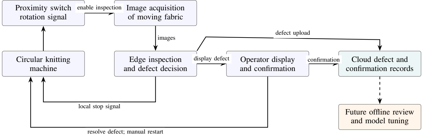
Fig. 1. Closed-loop inspection workflow for the circular knitting machine. Solid arrows describe the implemented production sequence provided for this study. The dashed cloud-to-review arrow represents offline data curation and later model tuning; it is not an online automatic-update claim. Hardware-specific timing and interlock details are intentionally not inferred and should be added from site measurements before submission.
