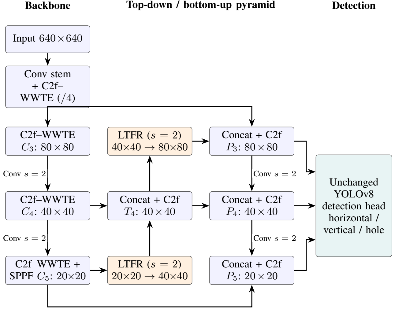
Fig. 3. Architecture of DACP-Net. C2f-WWTE replaces the four C2f refinement outputs in the backbone. LTFR replaces only the two top-down upsampling operations; the bottom-up fusion and prediction head follow YOLOv8n.
