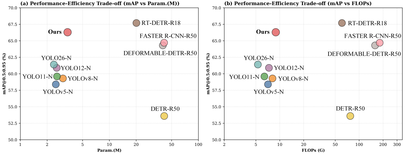
Fig. 5. Accuracy-efficiency trade-off of the retained test results. Both horizontal axes use a logarithmic scale. Marker coordinates are the exact values in Table II; the plot does not contain manual coordinate compression.
