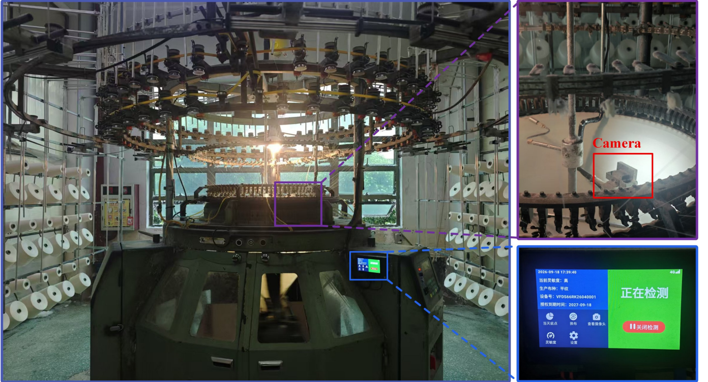
Fig. 2. Actual production-line installation on the circular knitting machine. The upper inset highlights the camera location; the lower inset shows the edge-side touch display while inspection is active. Colored callouts and insets are retained from the installation record.
