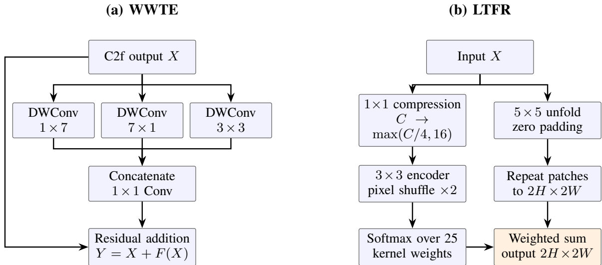
Fig. 4. Internal structures of (a) WWTE and (b) LTFR. WWTE uses three depthwise branches and residual fusion. LTFR generates location-specific 5 \times 5 reassembly kernels at scale 2.
