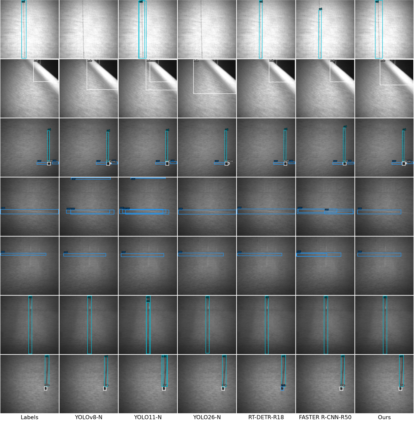
Fig. 5. Qualitative comparison on selected test images. Columns are labels, YOLOv8n, YOLO11n, YOLO26n, RT-DETR-R18, Faster R-CNN-R50, and DACP-Net. The figure uses a common renderer for visual consistency; it should be updated after finalizing the exact sample-selection protocol and display confidence threshold.
