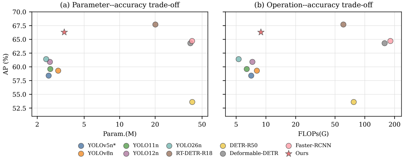
Fig. 4. Accuracy-efficiency trade-off of the retained test results. Both horizontal axes use a logarithmic scale. Marker coordinates are the exact values in Table II; the plot does not contain manual coordinate compression.
