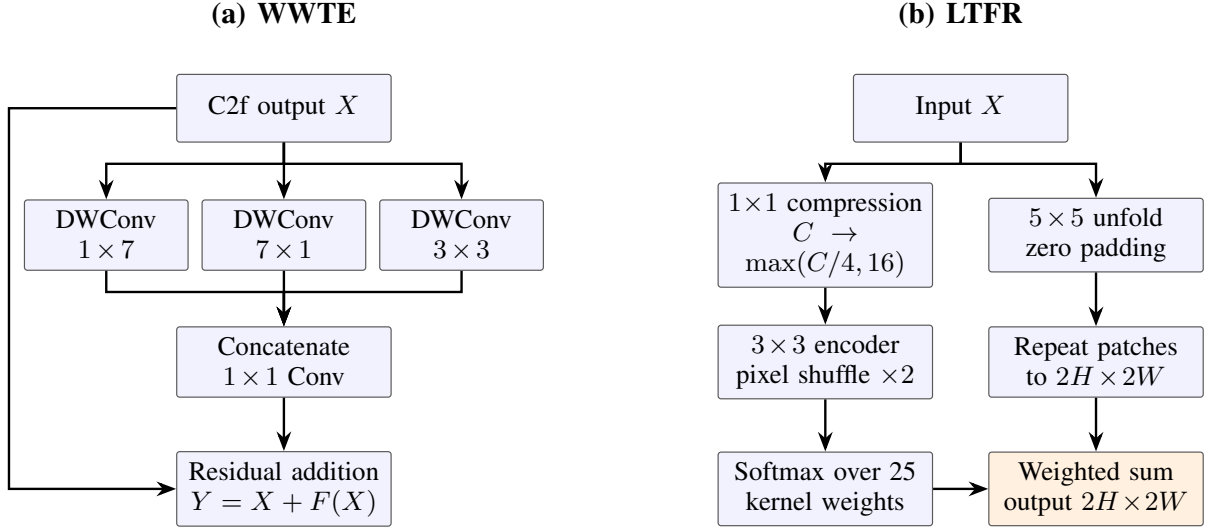
Fig. 3. Internal structures of (a) WWTE and (b) LTFR. WWTE uses three depthwise branches and residual fusion. LTFR generates location-specific 5 \times 5 reassembly kernels at scale 2.
