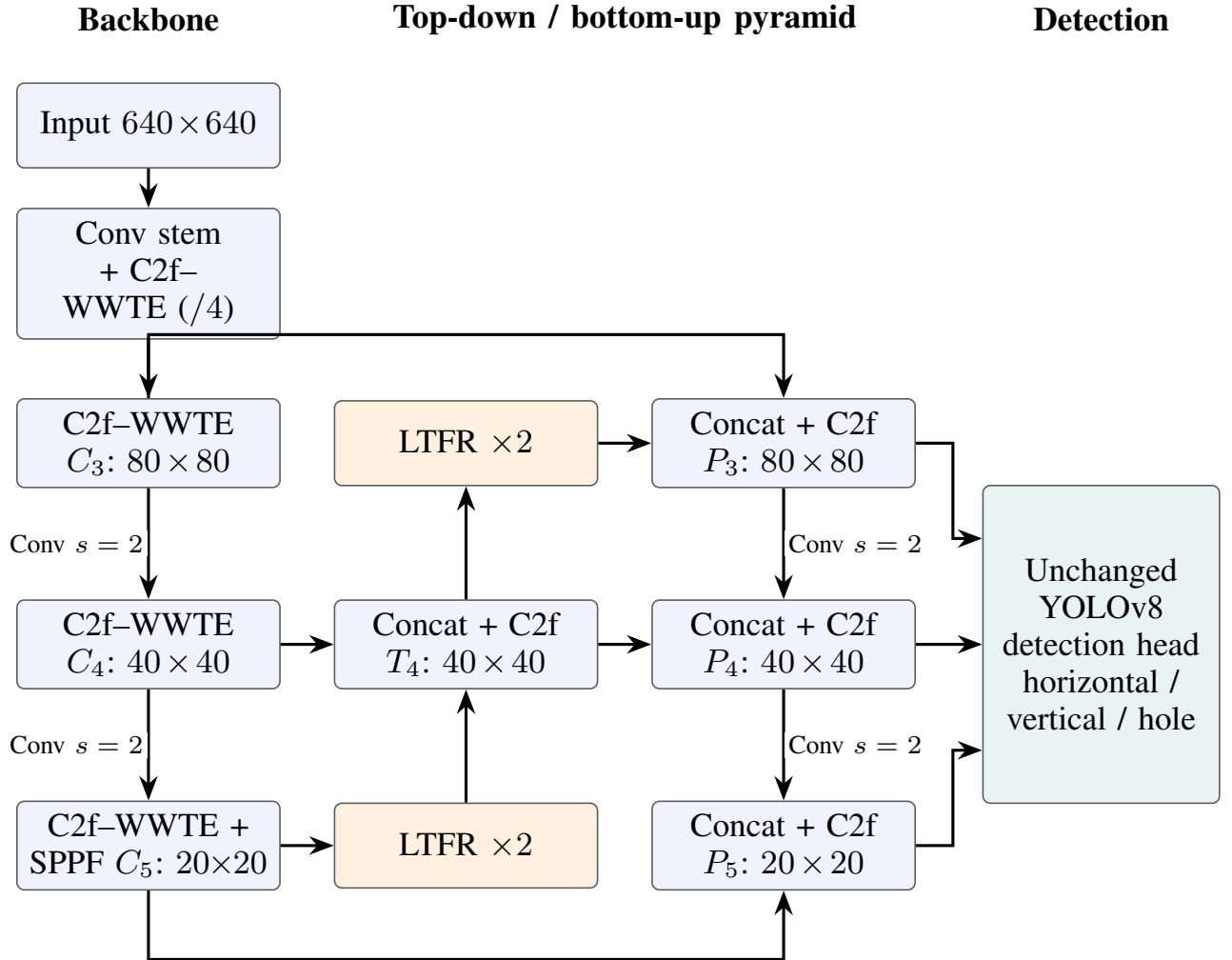
Fig. 2. Architecture of DACP-Net. C2f-WWTE replaces the four C2f refinement outputs in the backbone. LTFR replaces only the two top-down upsampling operations; the bottom-up fusion and prediction head follow YOLOv8n.
