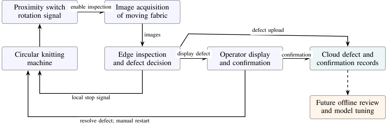
Fig. 1. Closed-loop inspection workflow for the circular knitting machine. Solid arrows describe the implemented production sequence provided for this study. The dashed cloud-to-review arrow represents offline data curation and later model tuning; it is not an online automatic-update claim. Hardware-specific timing and interlock details are intentionally not inferred and should be added from site measurements before submission.
