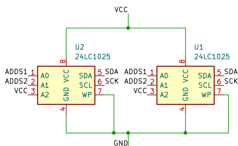
N3 - EEPROM
