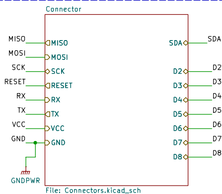
N4 - Connectors
