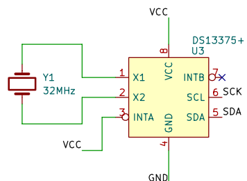
N1 - Clock/Calendar
