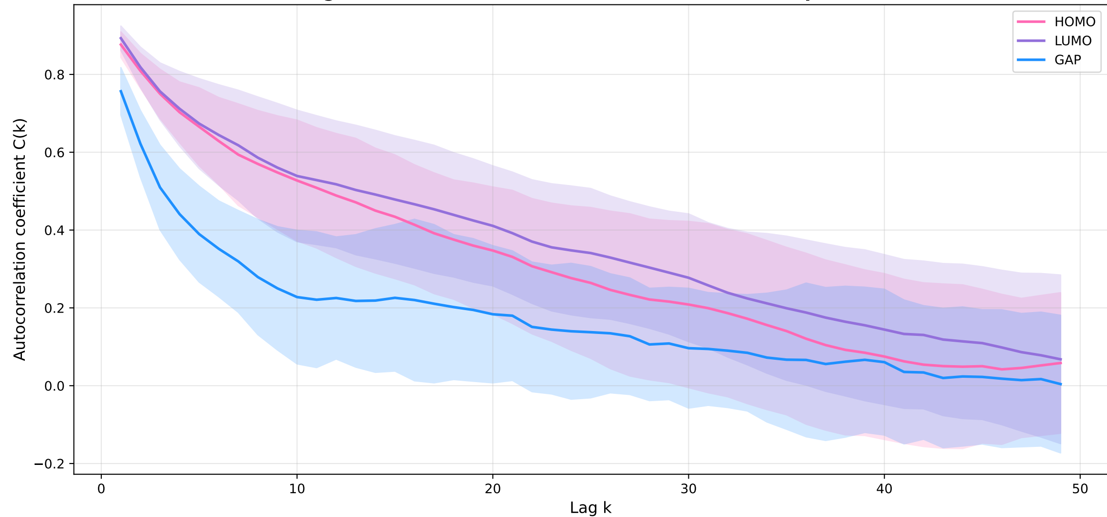
Average autocorrelations (HOMO, LUMO, GAP) for Experiment 3
