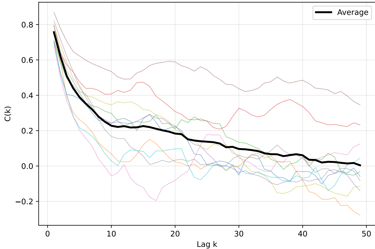
GAP - All autocorrelation for Experiment 3
