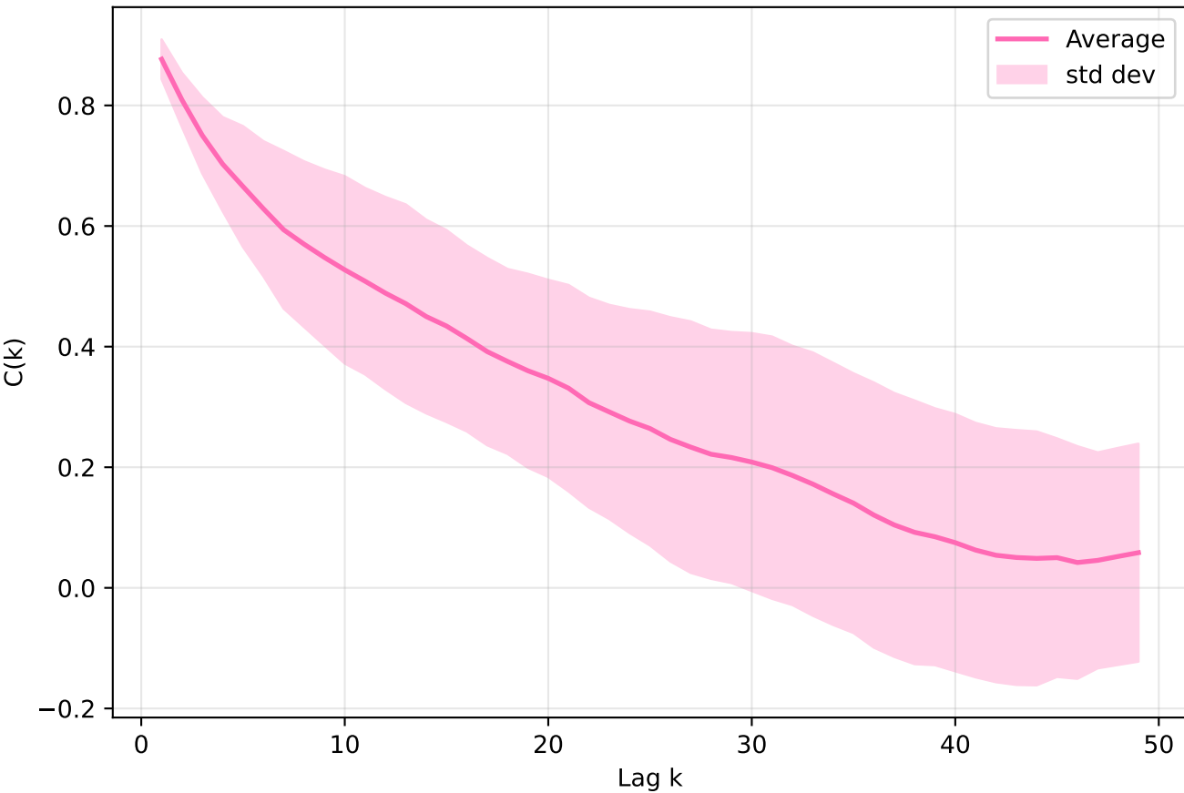
HOMO - Average autocorrelation for Experiment 3
