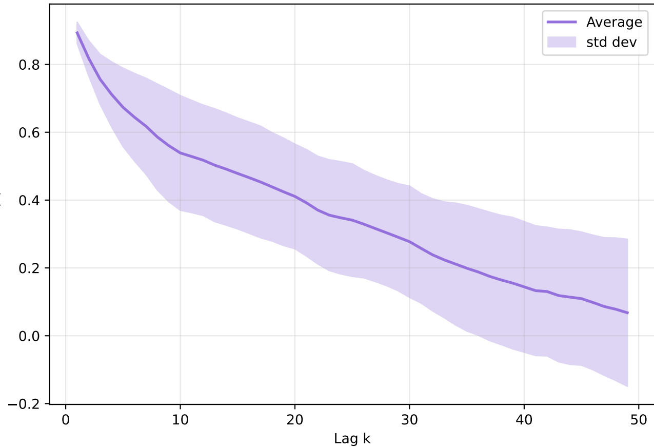
LUMO - Average autocorrelation for Experiment 3
