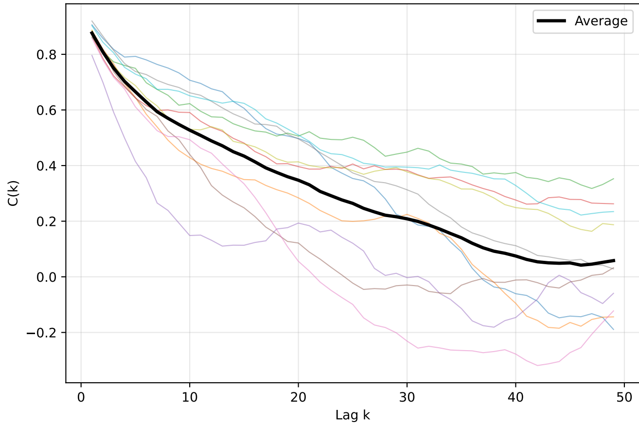
HOMO - All autocorrelation for Experiment 3
