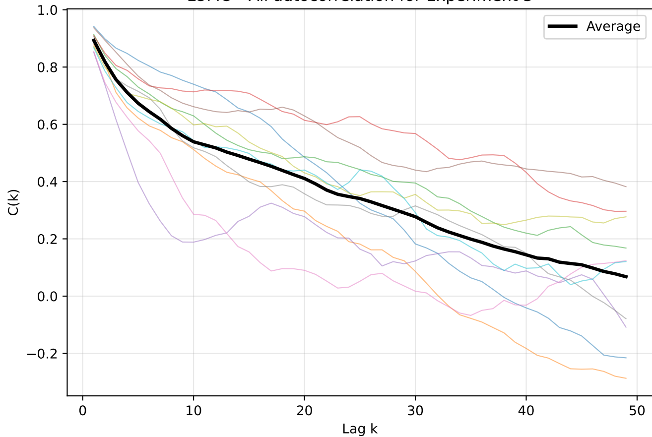
LUMO - All autocorrelation for Experiment 3
