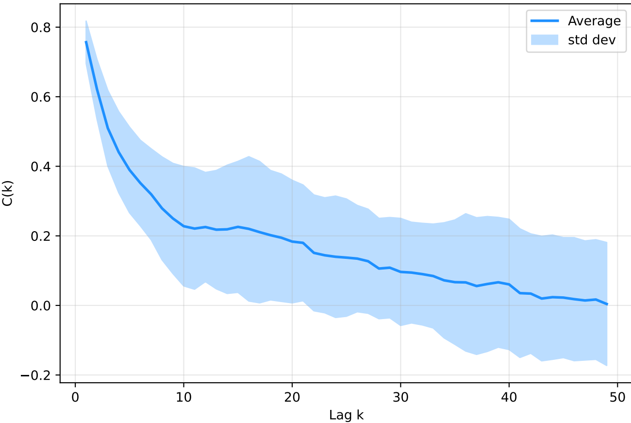
GAP - Average autocorrelation for Experiment 3
