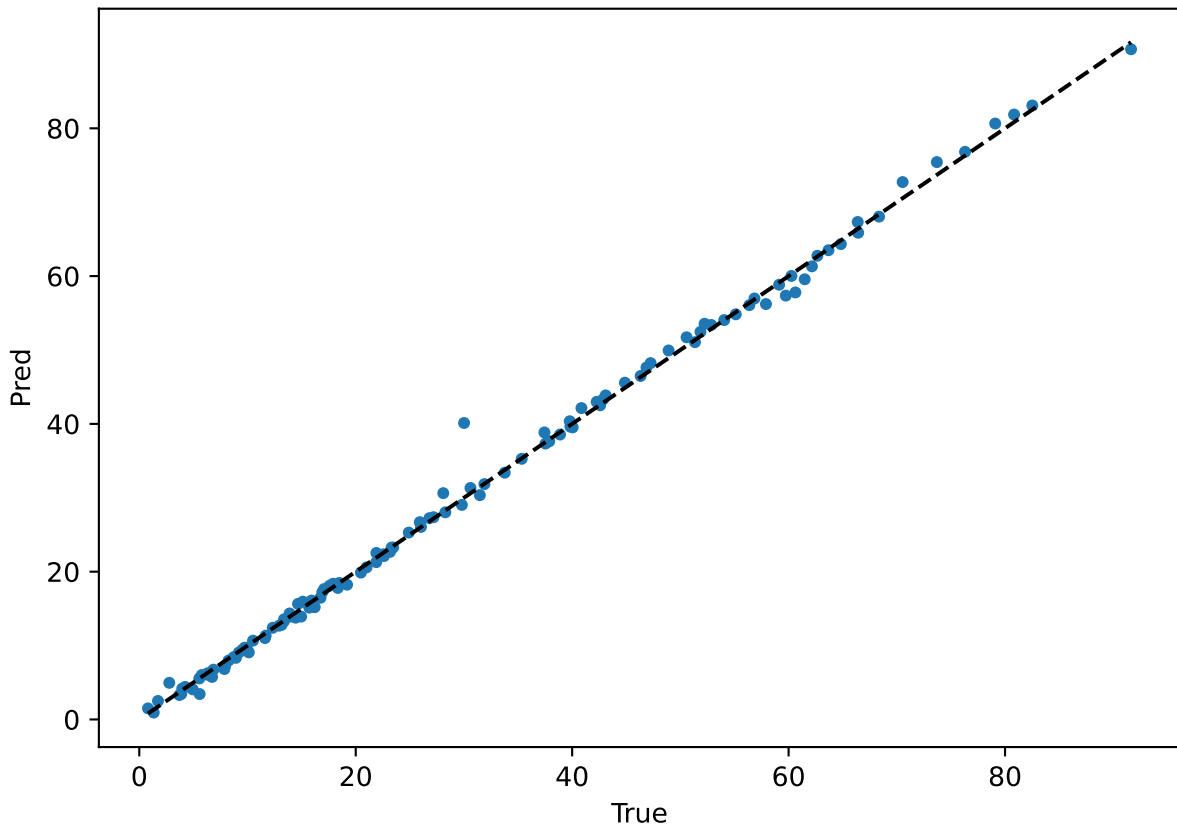
Branch Flow • Truth vs Prediction
