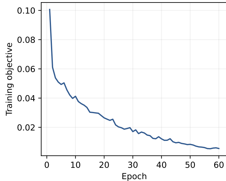
H3_mlp
