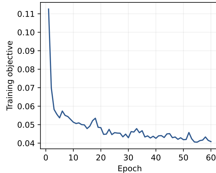
H3_linear
