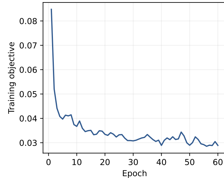
H32_linear
