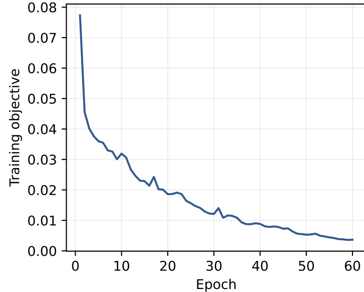
H32_mlp
