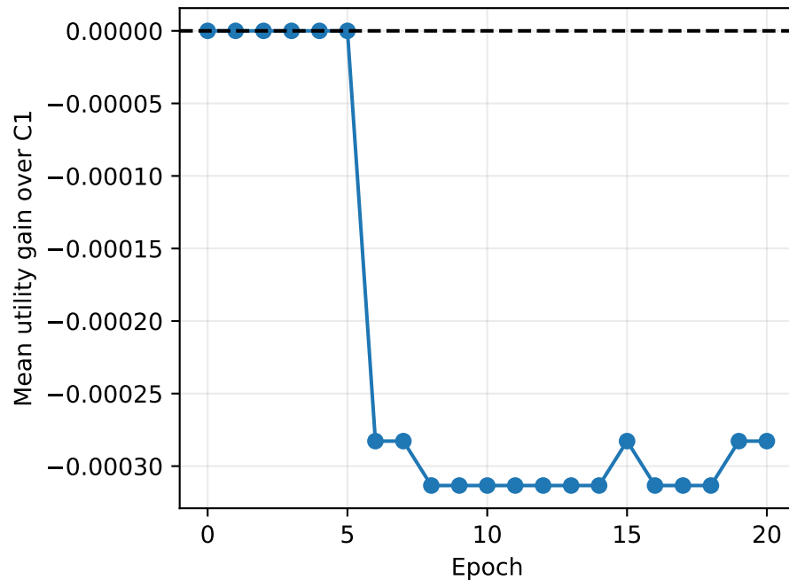
C3 v3: matched C1 initialization; TRAIN-held-out utility, not benchmark accuracy
