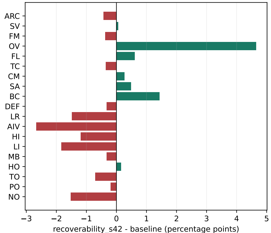
SR
