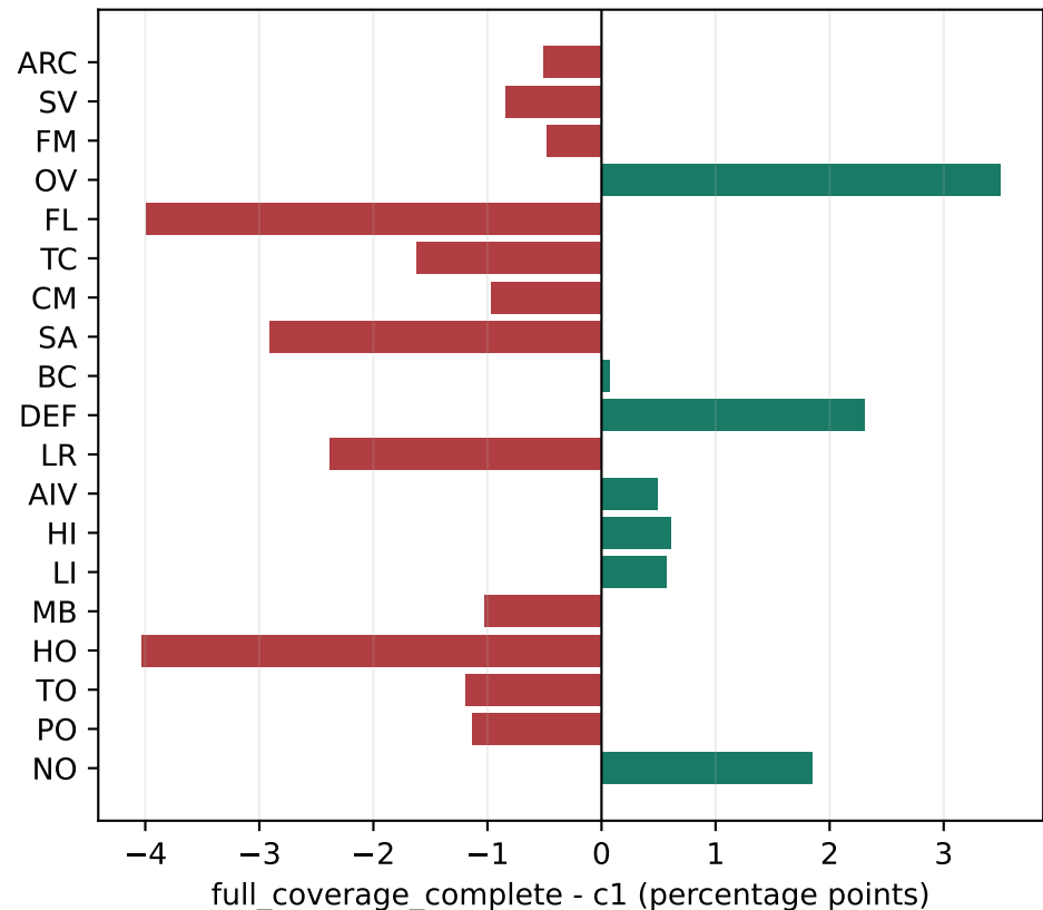
SR
