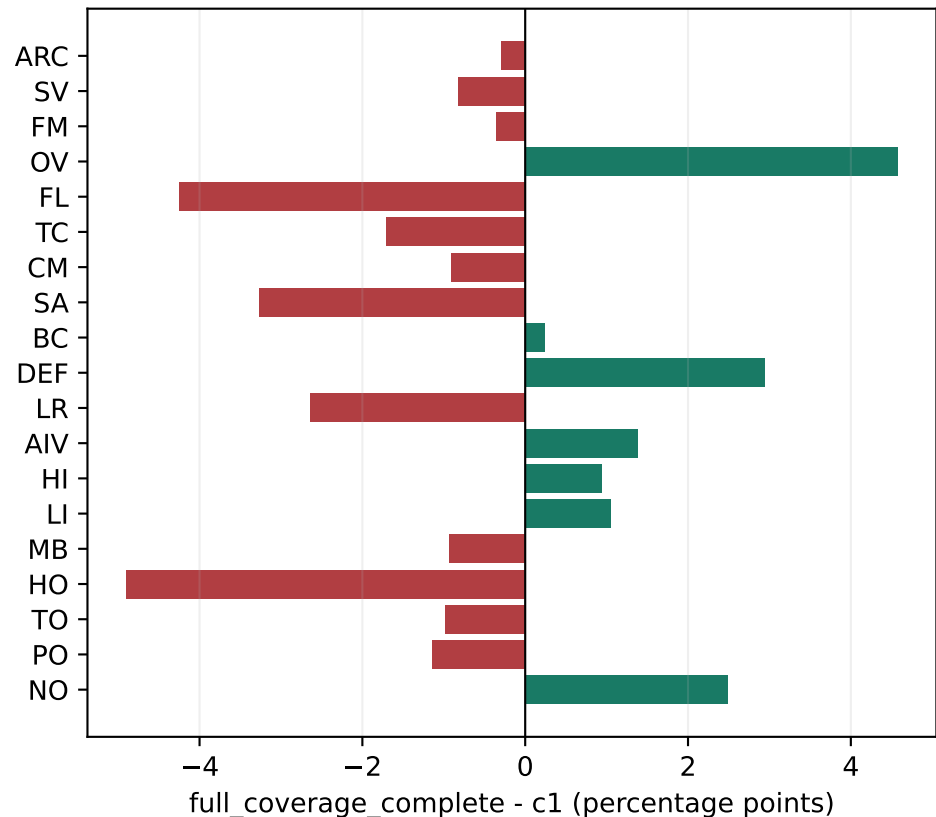
NPR
