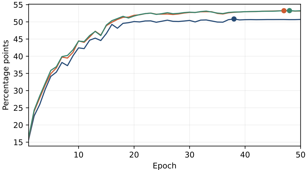
MSVR310 — mAP
