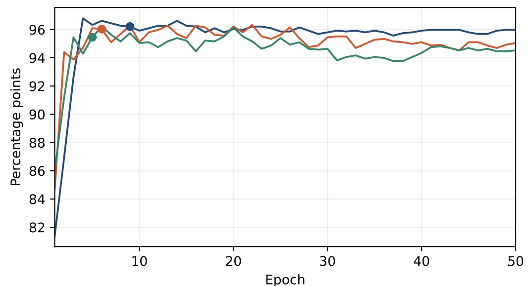
MSVR310 — Rank-1
