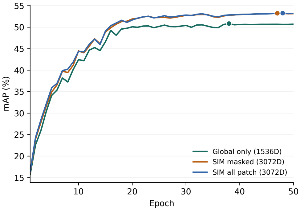
MSVR310: completed 50-epoch source references, seed 42 Dots follow each arm's mAP-best checkpoint
