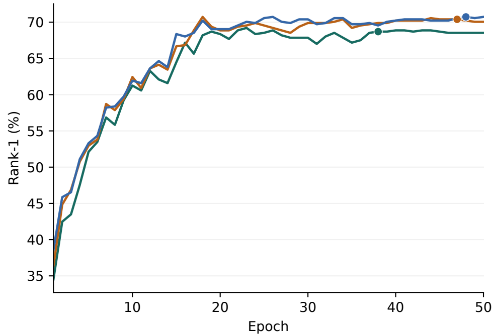
MSVR310: completed 50-epoch source references, seed 42 Dots follow each arm's mAP-best checkpoint
