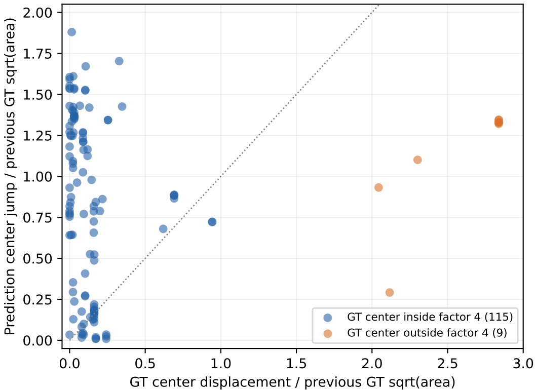
Motion: annotation versus tracker
