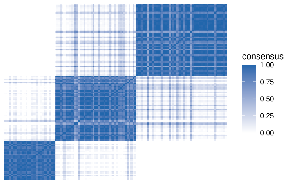
Consensus matrix (k=3)
