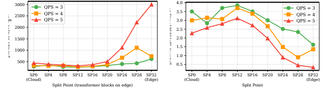
(a) Average latency across split points (b) 吞吐量 across split points
