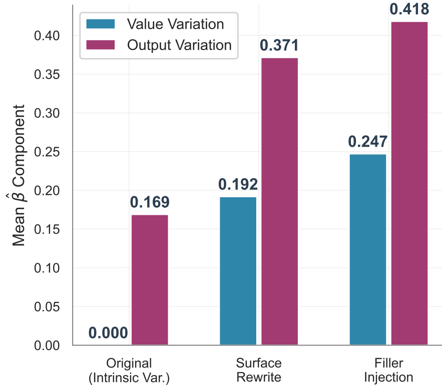
(b) \hat{\beta} Component Decomposition
