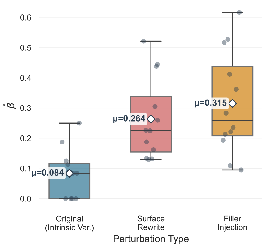
(a) Stability Under Semantic Perturbation
