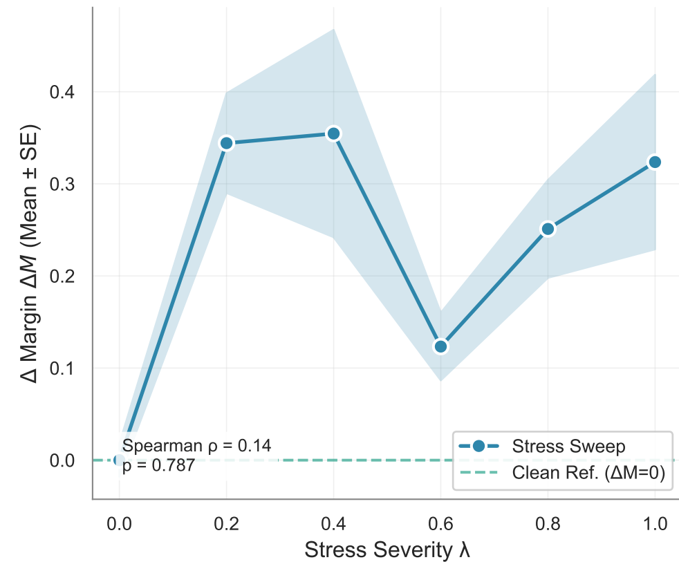
(a) Degradation from Clean Baseline
