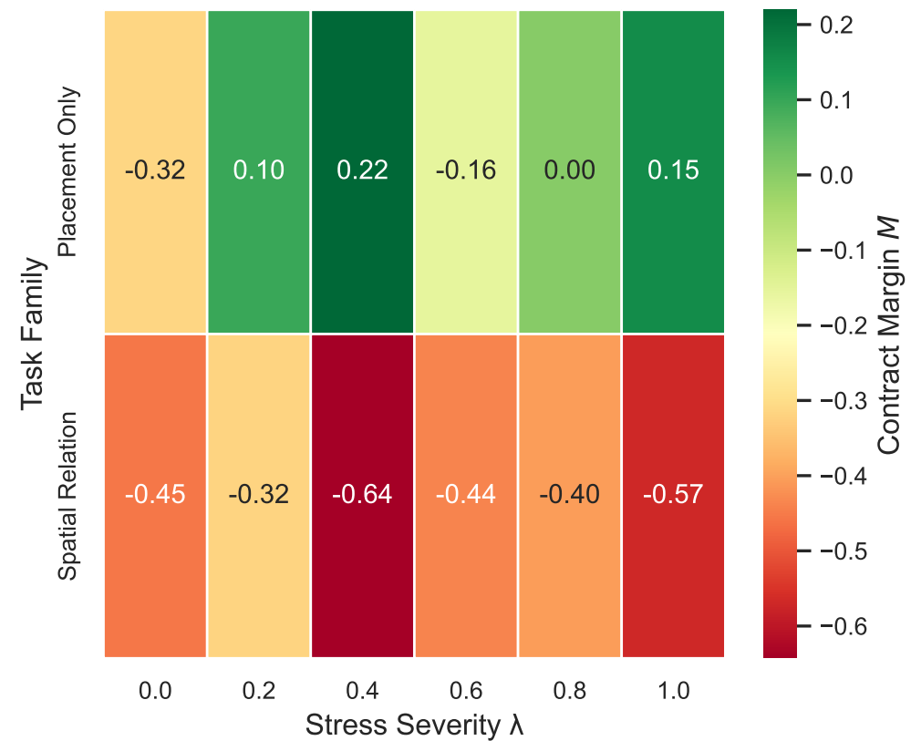
(c) Family-Specific Brittleness Heatmap
