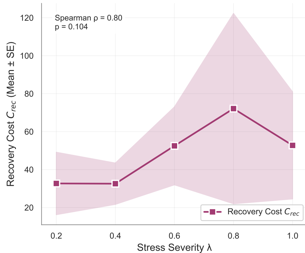
(b) Recovery Burden as Supporting Evidence
