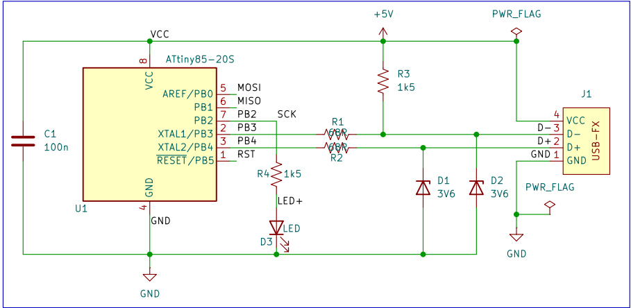
main circuitary
