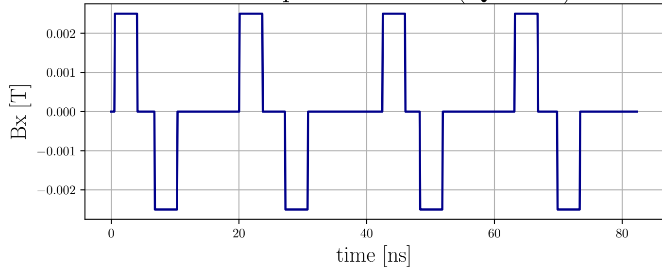
Pulse sequence for Bx (Qubit 0)
