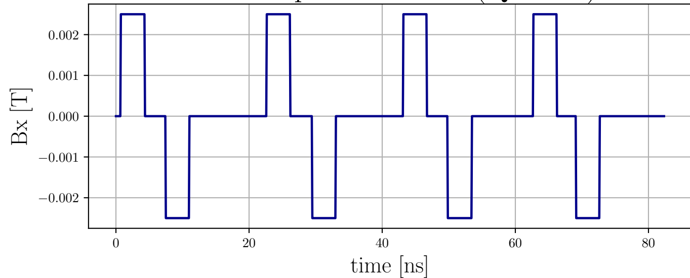
Pulse sequence for Bx (Qubit 1)
