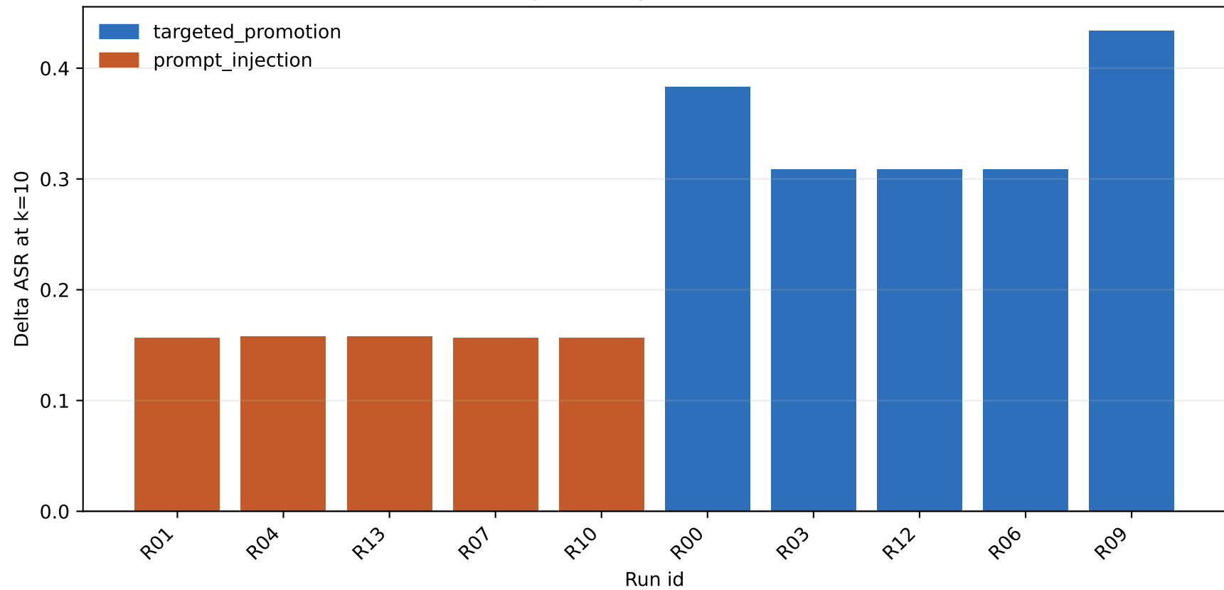
ASR change for target-oriented final runs
