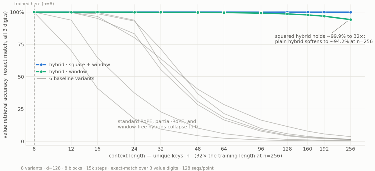
Figure 2: Exact-match retrieval accuracy (all 3 value digits) on second occurrences versus context length n (unique keys), 128 sequences per point. All variants are trained at n = 8 (dashed line) and reach \approx 100\% there. Only the windowed interleaved variants generalize: hybrid_square holds \sim 99.9\% to n = 256 (32 \times training length); plain hybrid declines to \sim 94.2\% . All six other variants (full RoPE, partial RoPE, and the window-free hybrids, with or without squared logits) collapse toward zero.
