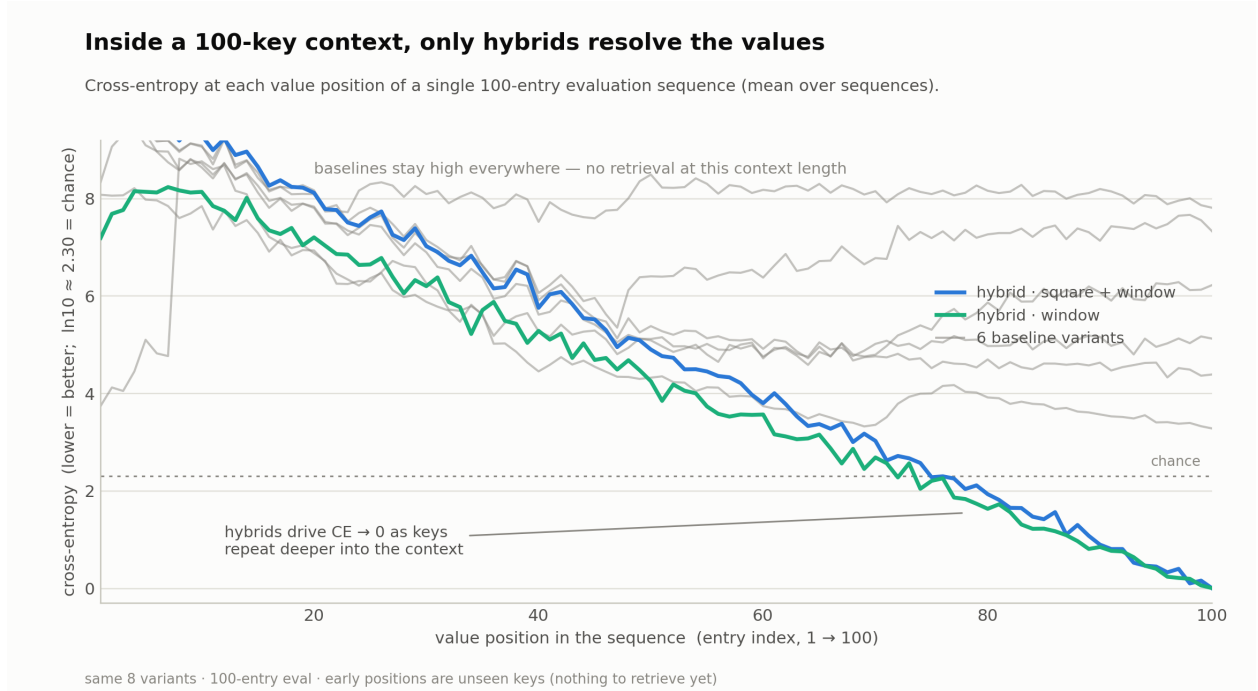
Figure 3: Mean cross-entropy per value digit at each entry index of a 100-entry evaluation sequence ( n = 50 keys, 12.5\times training length). Early entries are mostly first occurrences (nothing to retrieve), so all models sit above chance ( \ln 10 \approx 2.30 , dotted); as the sequence progresses, an increasing fraction of entries are second occurrences. Both windowed hybrids drive CE toward 0 deep into the context; the six baselines never descend below chance at any position: they perform no retrieval at all at this length.
