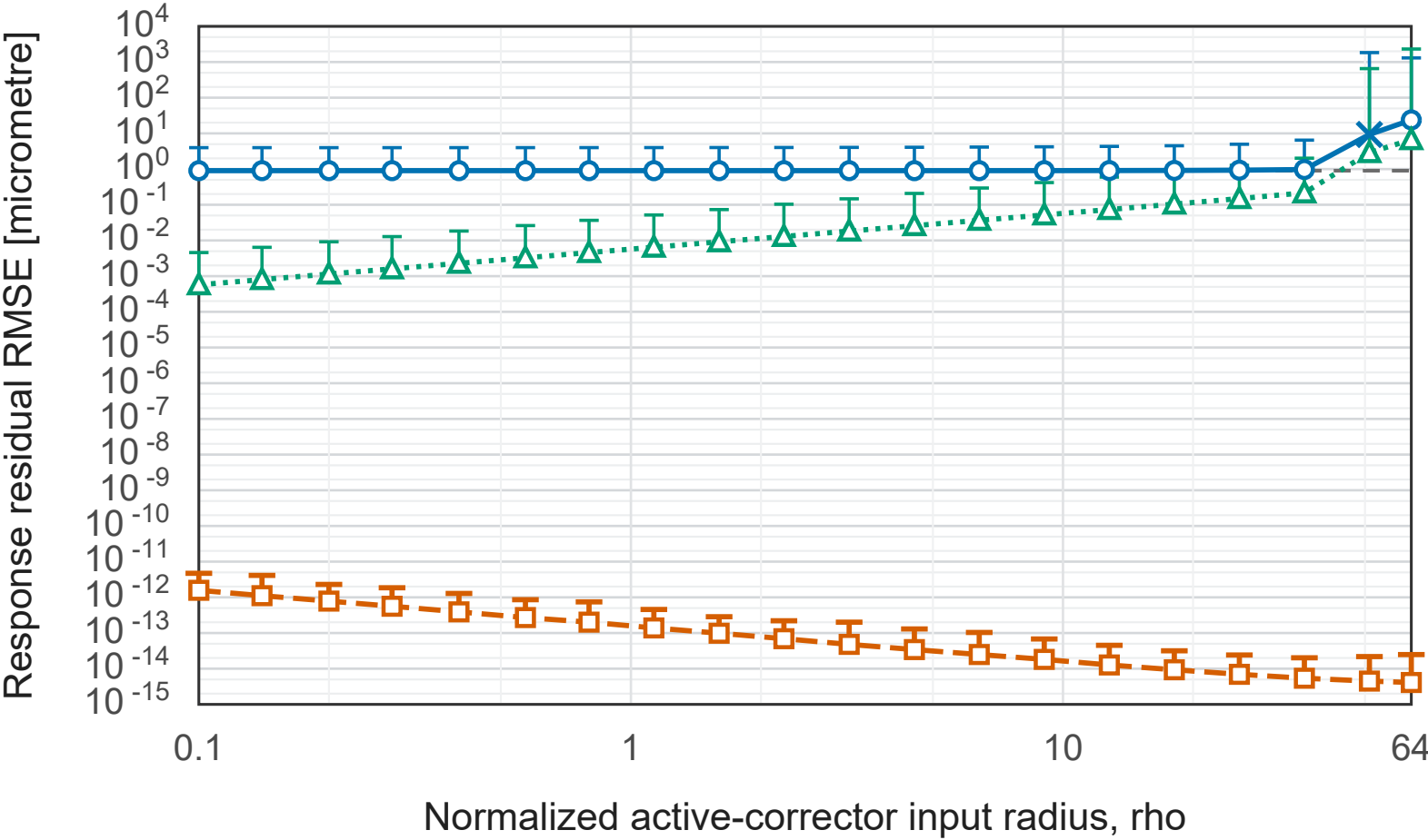
(b) Vertical detector orbit
