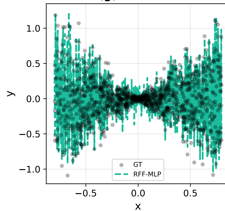
(g) RFF-MLP
