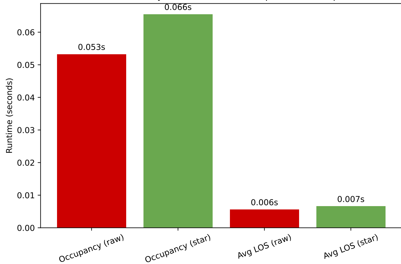
Raw vs Star Query Performance (two representative queries)
