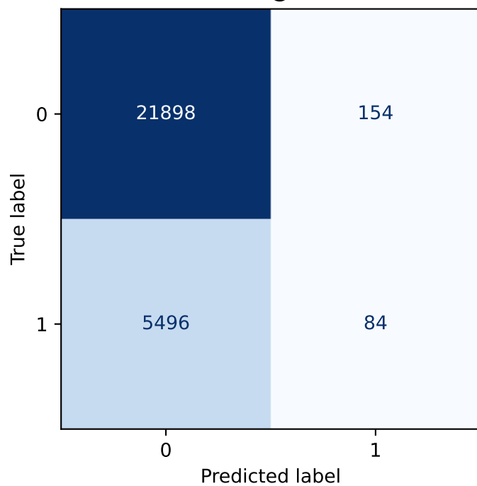
Confusion matrix @ threshold = 0.5
