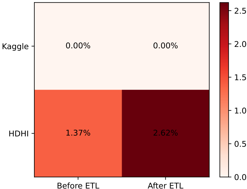
Average Missing Values (%) — Before vs After ETL
