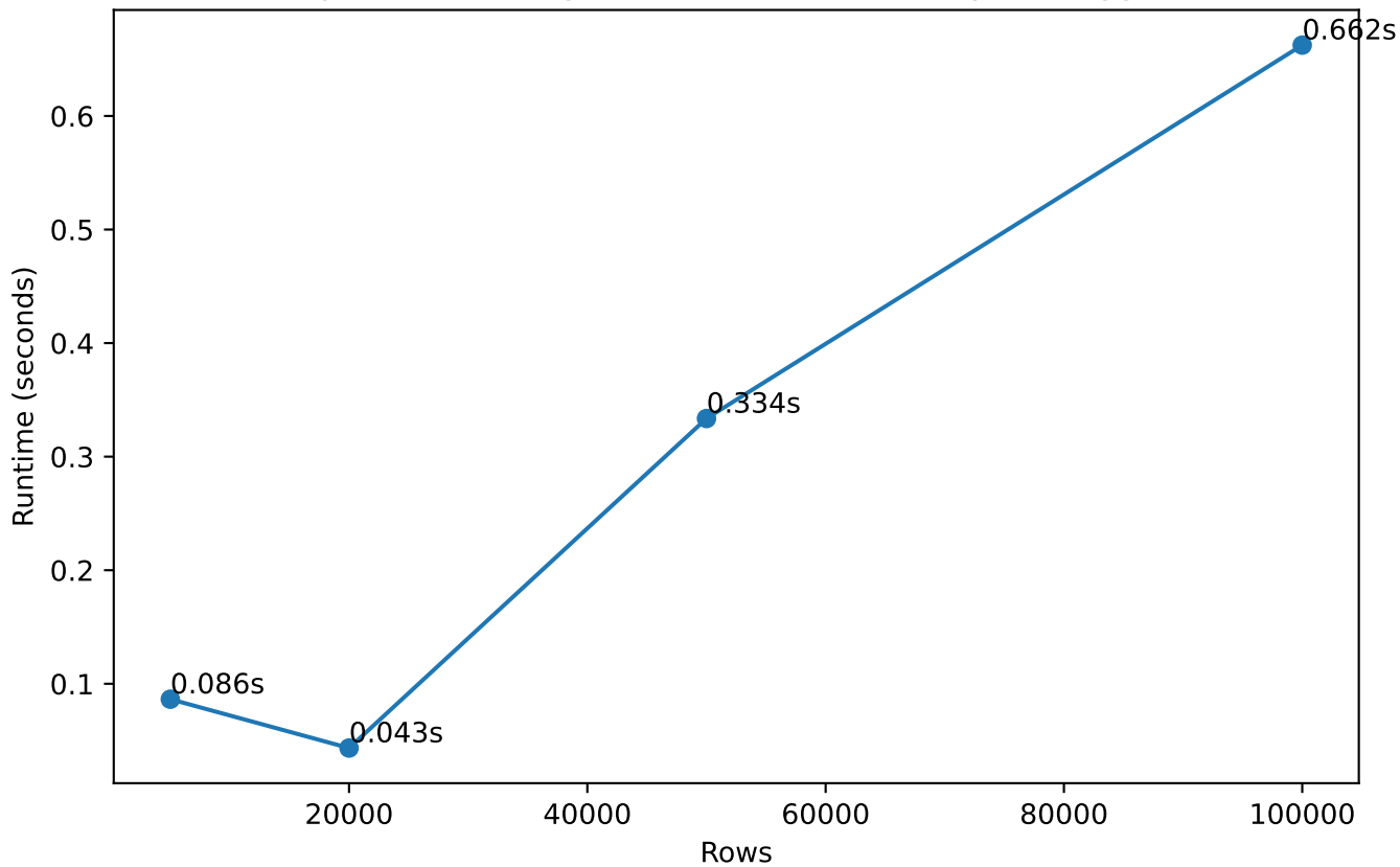
Pipeline Cleaning Runtime vs Rows (sampled Kaggle)
