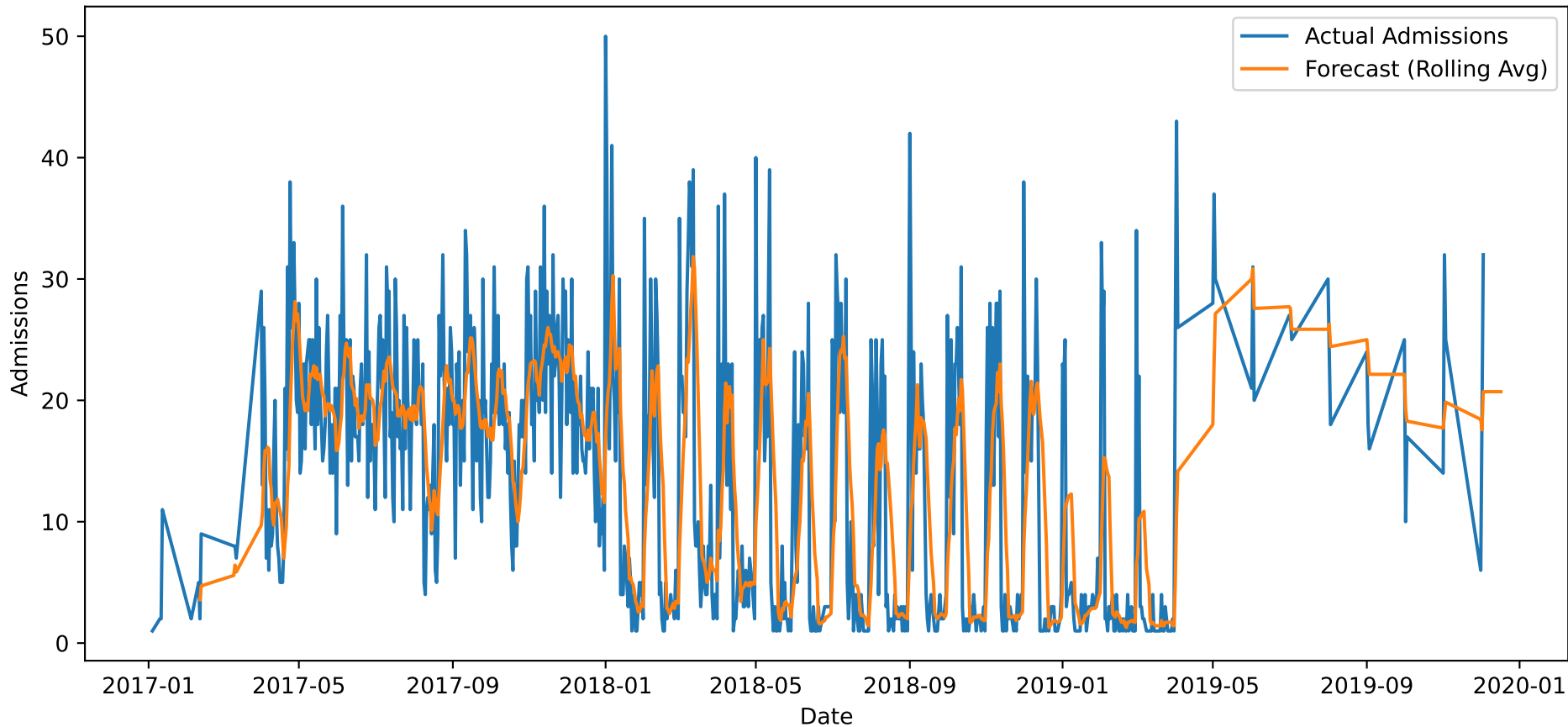
Actual vs Forecasted Hospital Admissions
