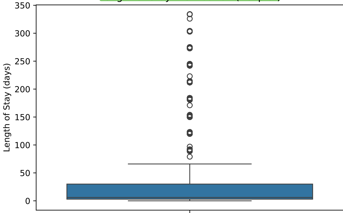
Length of Stay Distribution (Boxplot)
