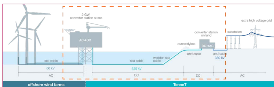
Figure 1: Offshore-to-mainland HVDC transmission and conversion corridor for a standardised 2 GW connection concept. Source: adapted from TenneT
