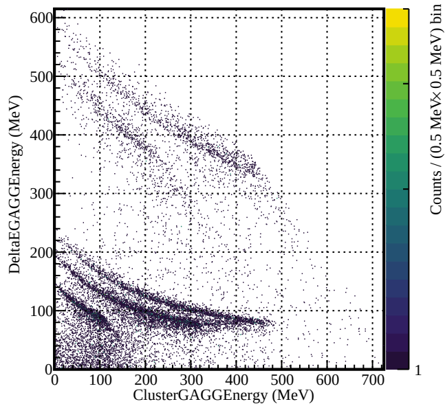
TOGAXSI \Delta E -E correlation
