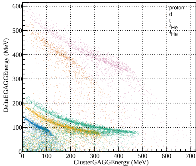
TOGAXSI \Delta E -E distribution by true PID
