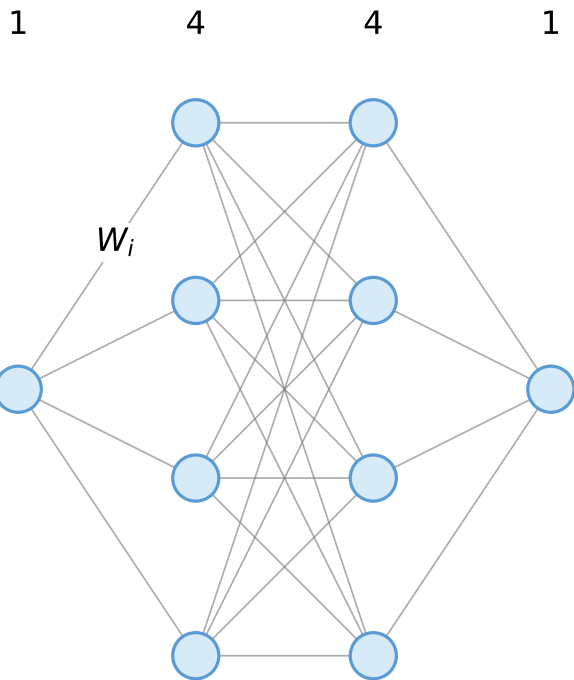
Multilayer Perceptron (MLP)
