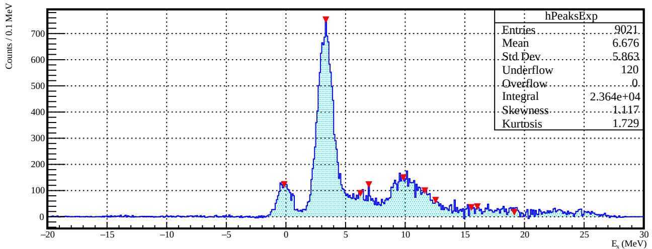
Background-subtracted excitation-energy spectrum
