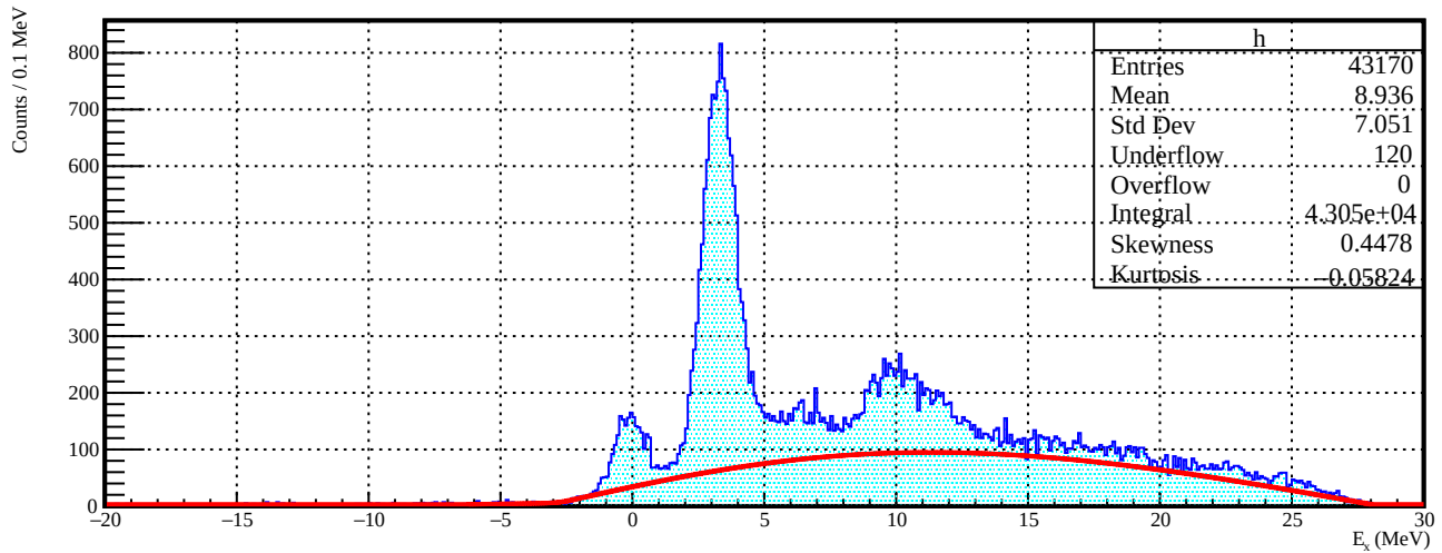
Experimental excitation-energy spectrum
