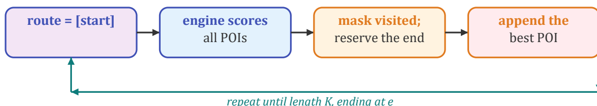
Figure 3 — Strategy A: build the route one POI at a time by rolling out the engine. Always loop-free, exactly K stops, \text{start} \rightarrow \dots \rightarrow \text{end} .
