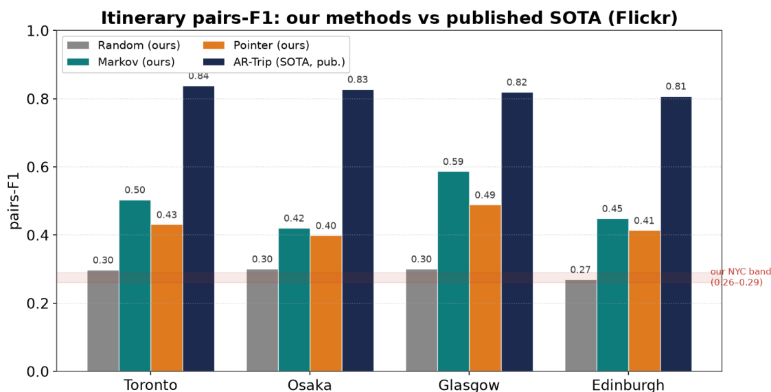
Figure 5 — Our methods beside the published SOTA. Strategy D validates the approach; it does not replace the headline engine + Strategy A.
